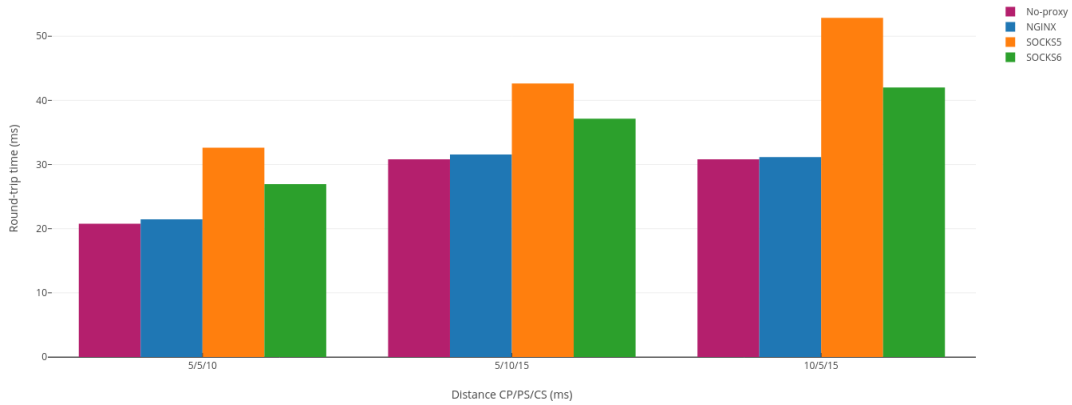
(a) The average of the client to server 120 consecutive requests round-trip time (ms) with changing configured distances between nodes.
